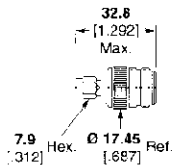
Part No. 1057381-1 M/A-COM Model No. 3082-2241-00
