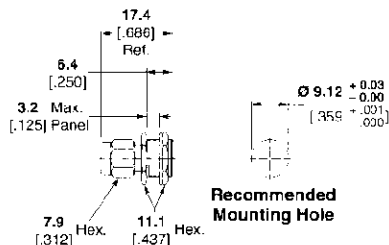
Part No. 1059758-1 M/A-COM Model No. 4585-2241-02
