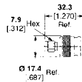
Part No. 1058664-1 M/A-COM Model No. 3682-2241-00
