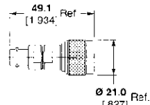
Part No. 1057390-1 M/A-COM Model No. 3082-2320-00
