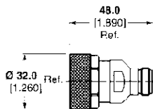
Part No. 1311205-1 M/A-COM Model No. A55P21E998X
